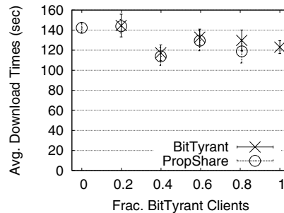
Figure 9: PropShare vs. BitTorrent
