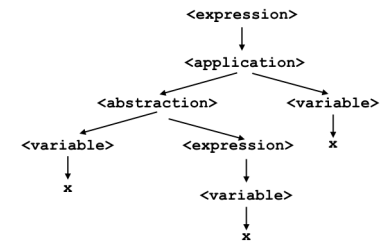
Figure 11: Incorrect derivation of the expression \lambda x . xx .
