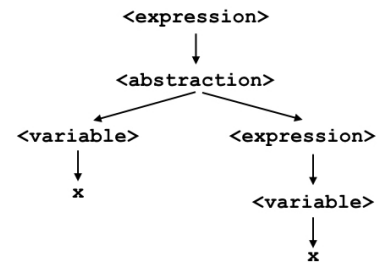
Figure 8: Derivation of the expression \lambda x. x .
