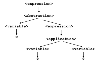
Figure 10: Correct derivation of the expression \lambda x . xx .
