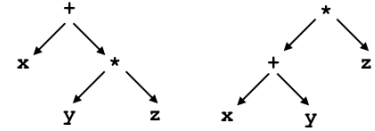
Figure 9: Without precedence, you'd have multiple derivations of the expression x + y * z . The left derivation is the one we want.
