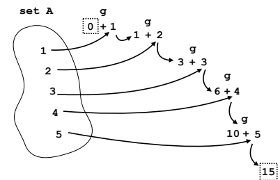
Figure 15: g is defined as fun acc x -> acc + x . When given the folding function g , the set A , and the initial value 0, the fold operation yields 15.
